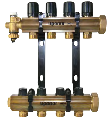
TruFLOW Jr. and Classic assemblies with balancing and isolation valves
