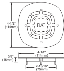
2" Stainless Steel Strainer Plate STRWL000 — $31
